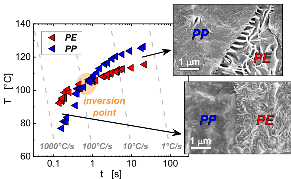
Figure 1. Continuous Cooling Curve diagrams for PE and PP phase in a blend and morphology at different cooling conditions.
